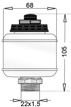
SOF26 Con sensore livello olio With oil level check control
