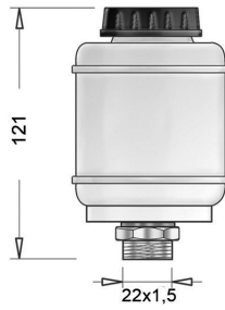
SOF19M Serbatoio olio minerale Mineral oil tank SOF19 Serbatoio olio freni DOT DOT brake oil tank
