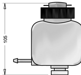
SOF14 Con sensore livello olio With oil level check control TA26343 Serbatoio olio minerale Mineral oil tank
