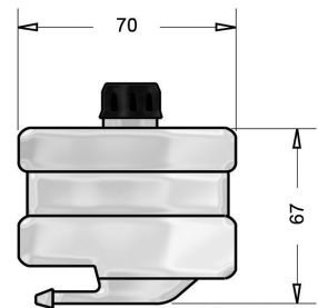
SOF15 Serbatoio olio freni DOT DOT brake oil tank Z657 Staffa supporto serbatoio Oil tank bracket
