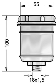
SOF11 Serbatoio olio freni DOT DOT brake oil tank
